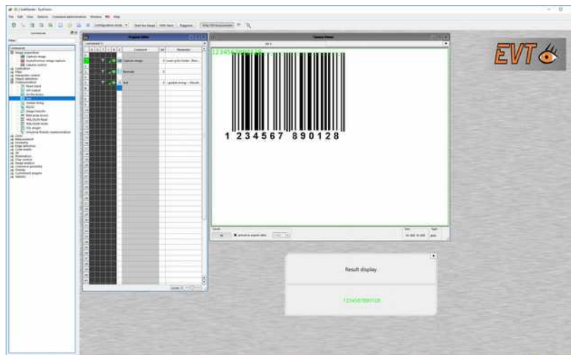
EyeSensN Configuration Mode: bar code reading
